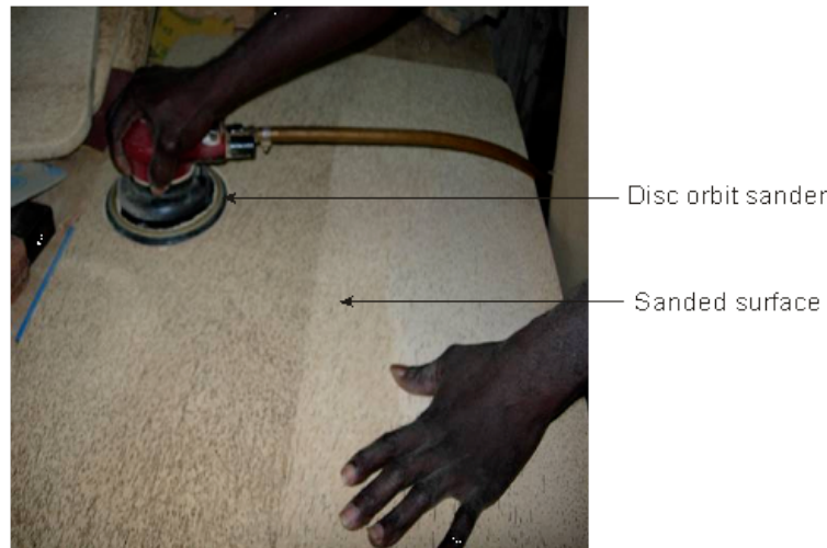
Fig 1. Orbital sanding of oil palm lumber
